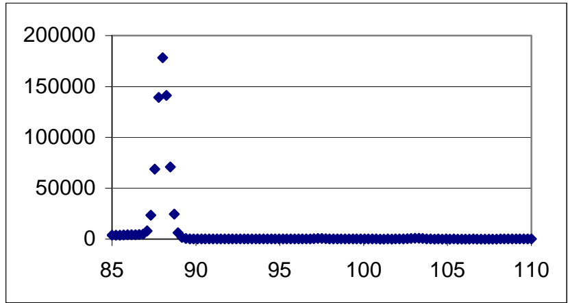
Figure 12: Spectrum for the ^{109}\text{Cd} source used during sample measurement, shows contamination peaks an order of magnitude smaller than the 88keV peak
