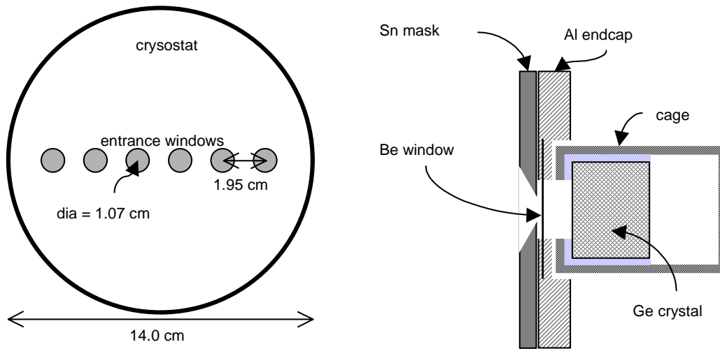
Figure 7: Narrow collimation, (left) view of detector array with six beryllium windows and (right) collimating tin mask and the detector housing (Evans, 1999)
