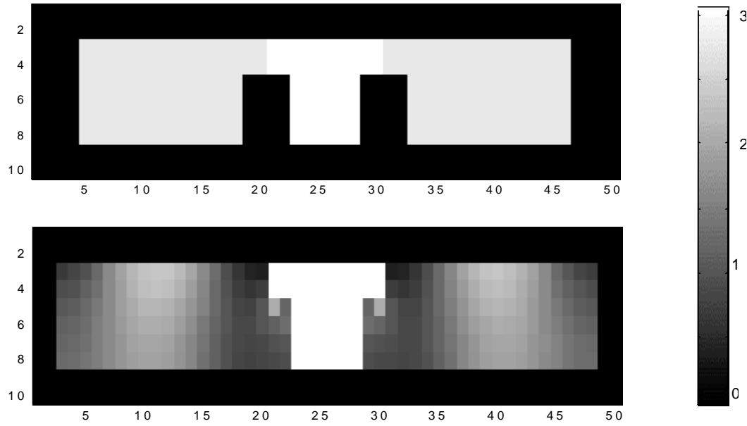
Figure 27: 2D projection of electron density map (Top) plot of actual sample and (bottom) reconstruction from measured data, assuming top and bottom boundary is known, x and y-axis map voxel coordinate while shade indicates density value
